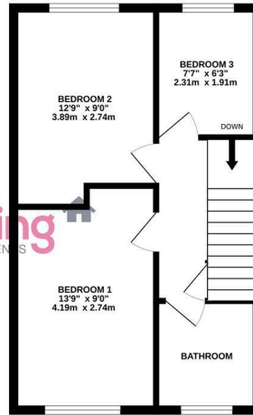
1ST FLOOR 399 sq.ft. (37.0 sq.m.) approx.
